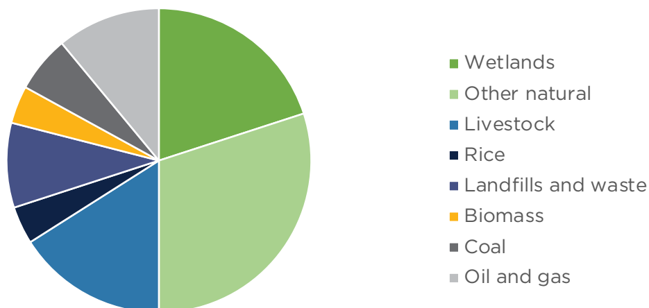
Figure 1: Global inventory of methane emissions
